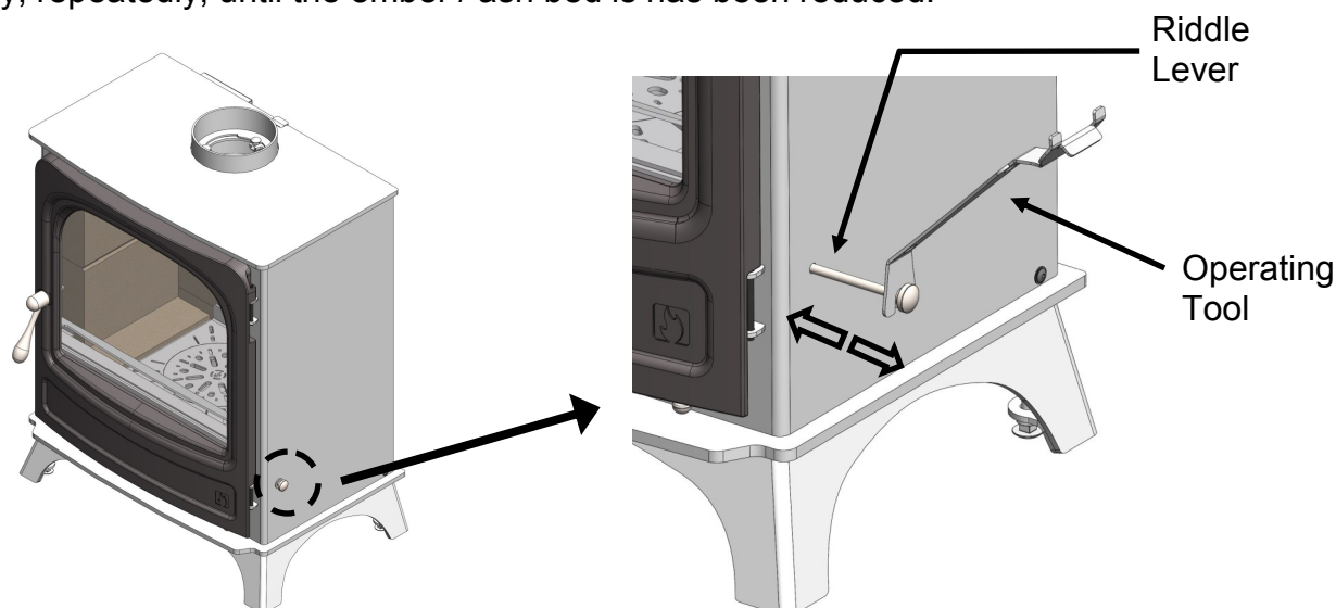
Fig. 6. Riddle Lever
